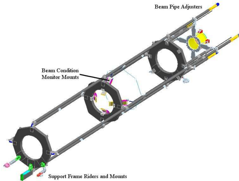
Figure 21. Illustration of the Beam Pipe Support Structure as described in the text.
