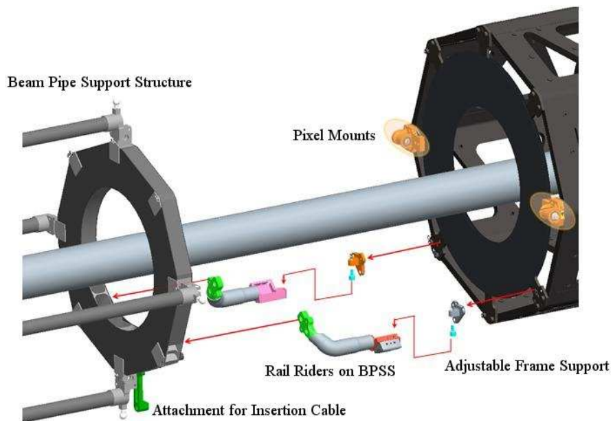
Figure 21. Illustration of the Beam Pipe Support Structure as described in the text.
