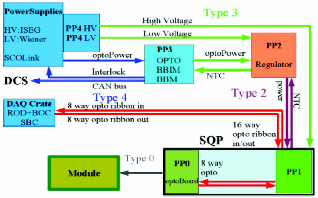
Figure 7.1.3 Schematic of the pixel electrical and optical services. ****Placeholder****
