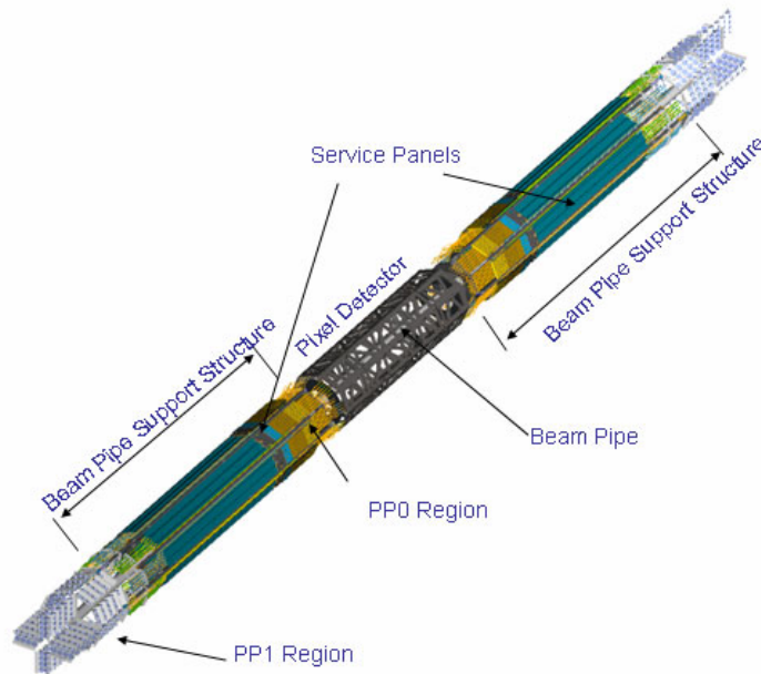
Figure 7.1.1 A perspective view of the pixel detector and internal services. ****Placeholder****
