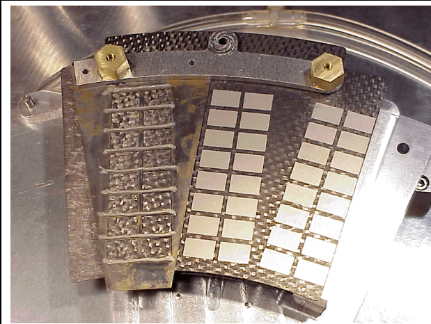
Figure 31. Example of screening CGL-7018 on to sector.
