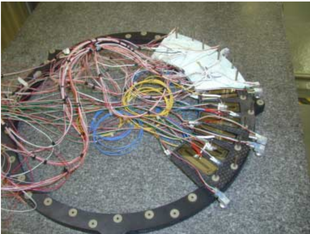
Figure 33. Second prototype disk using sealed-tube sectors under assembly at HYTEC, Inc.
