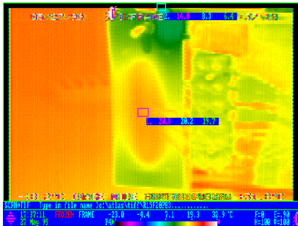
Figure 18. Test piece after 50 MRad and after pressure cycling to 4 bar absolute 20 times.
