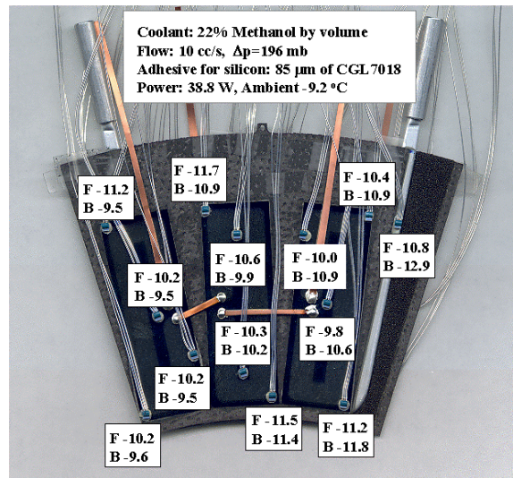
Figure 11. Typical results of measurements at low temperature, and after temperature cycling. Inlet fluid temperature was -15^{\circ}\text{C} . F => front and B => back of sector.
