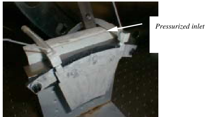
Figure 24. Photograph of HYTEC sector pressure test setup. Inlet tube at upper right is open to pressure source. Exit tube at the left is sealed to prevent flow during the test.
