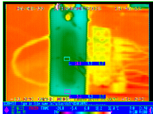
Figure 19. Test piece after all stress testing with 5°C water/methanol coolant at 10 cc/sec - see text.
