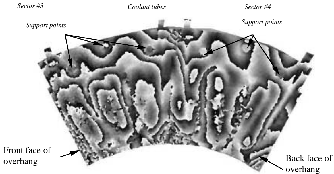
Figure 21. Phase map of fringe pattern illustrating out-of-plane distortions from power off to power on condition. Power state of 18W, with room temperature coolant at 9 cc/sec.
